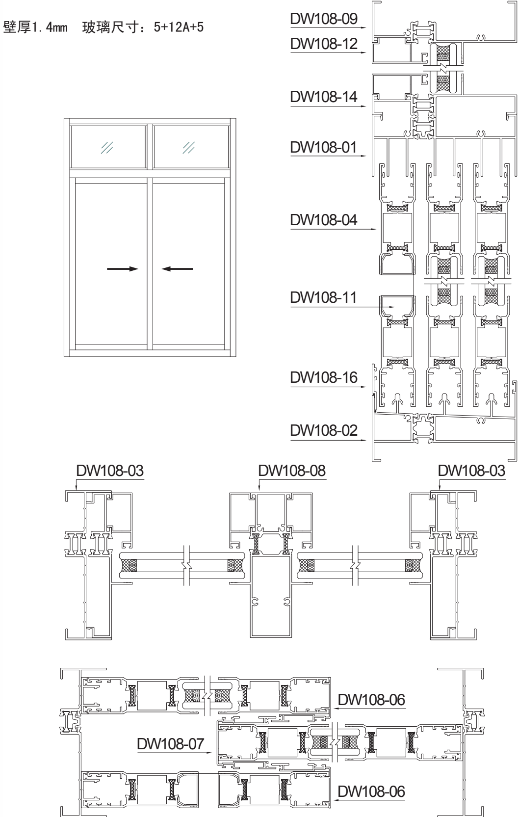
HL-DW108 three panels sliding window series
