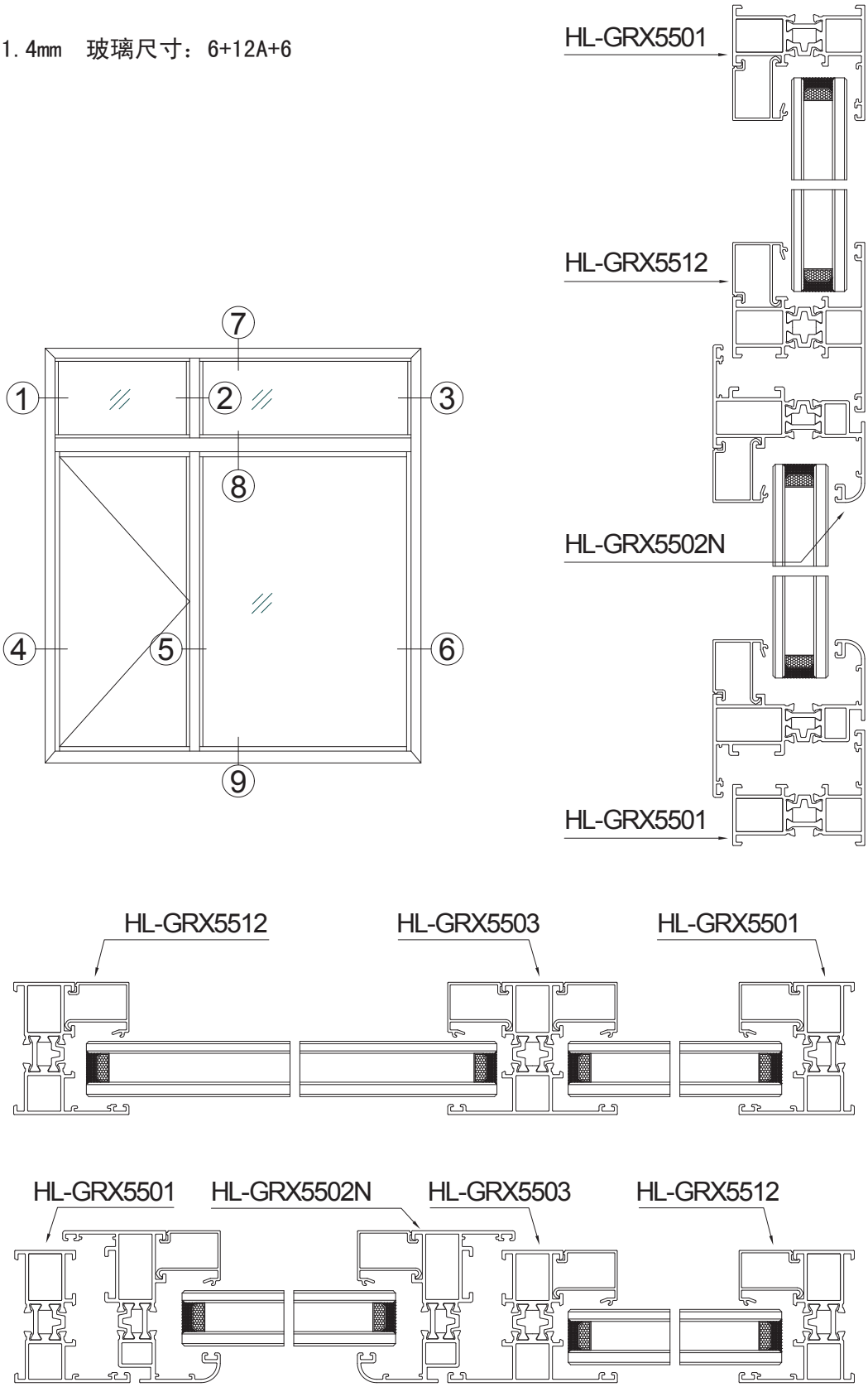
HL-GRX55 casement window series
