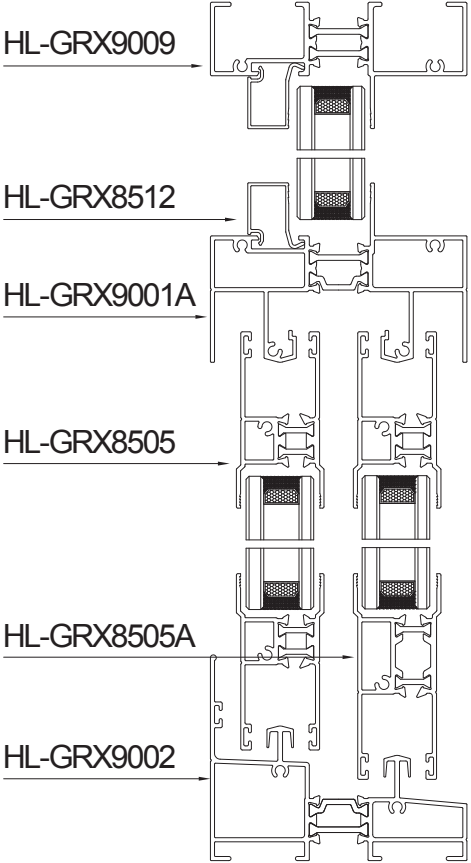
HL-GRX908 sliding door, window series
