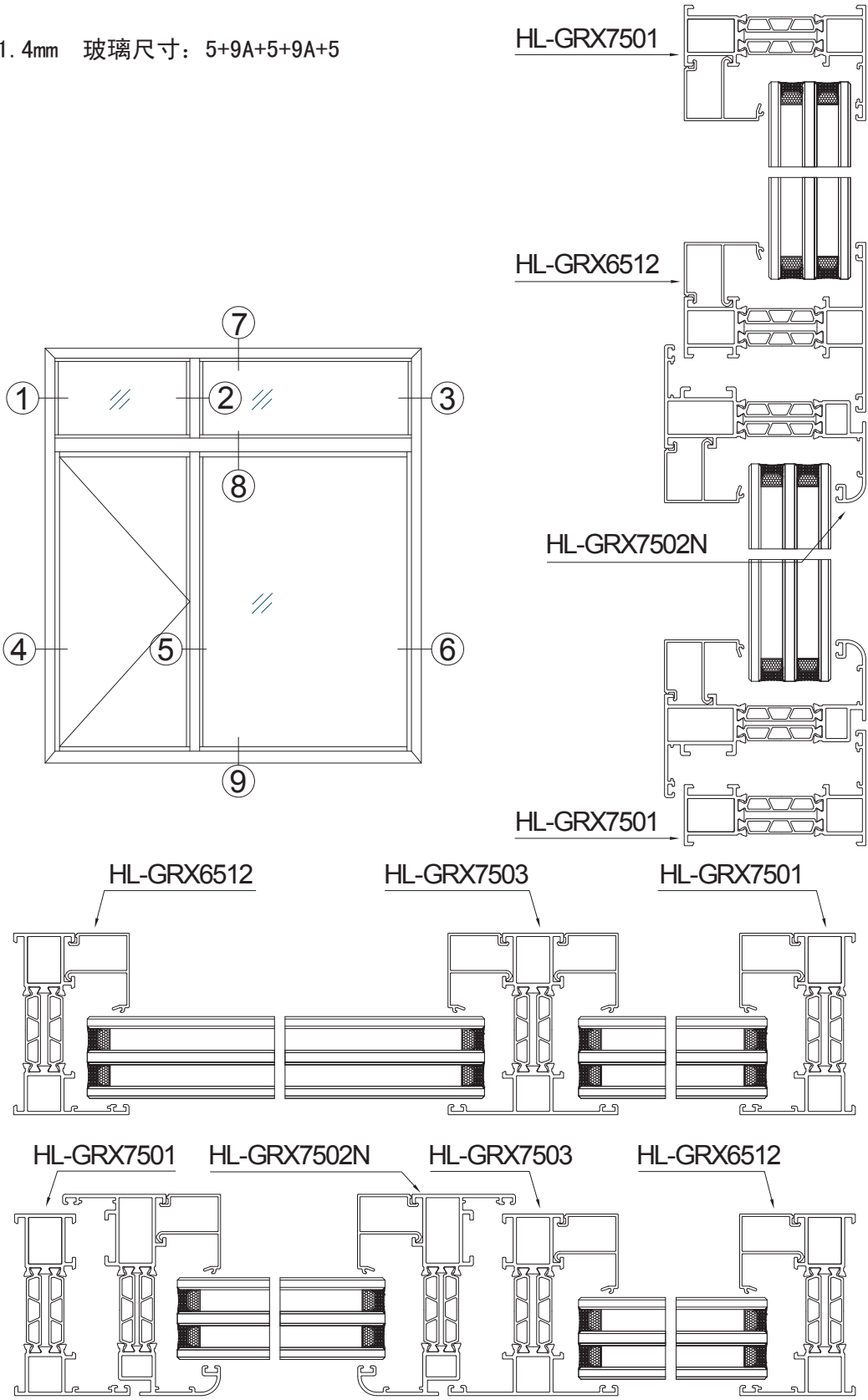
HL-GRX75 casement window series
