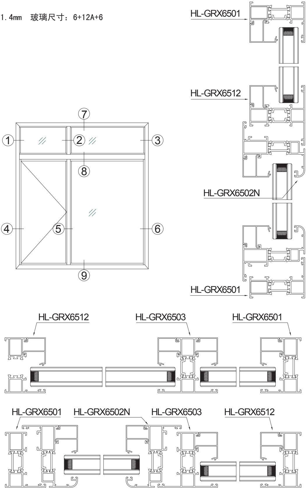
HL-GRX65 casement window series
