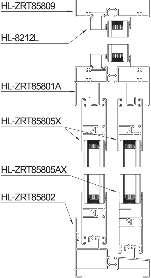
HL-858 injection thermal break sliding window series
