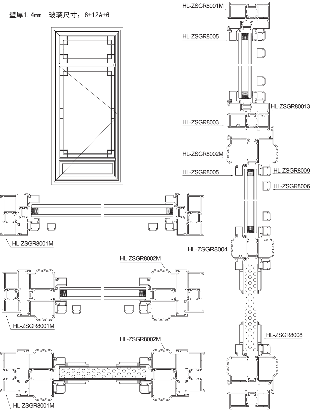
Huiyun series Chinese window No.2
