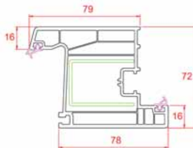
Narrow Door Sash
