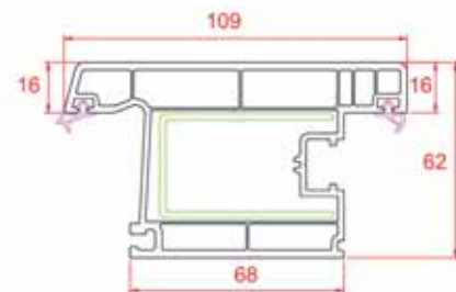
Outward Door Sash
