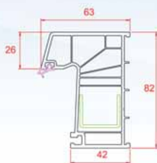
Frame
