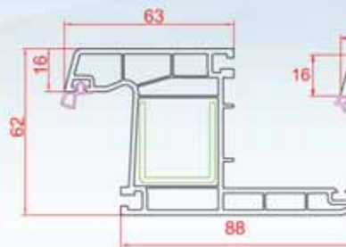
Wide Architrave Frame
