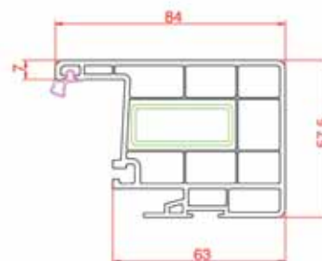
Mullion
