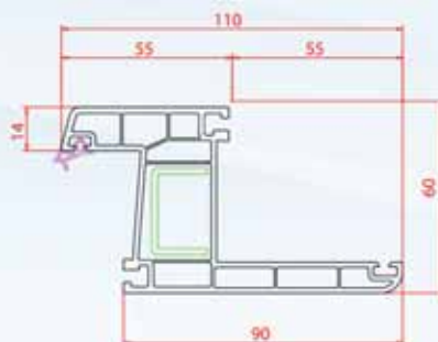
Architrave Frame
