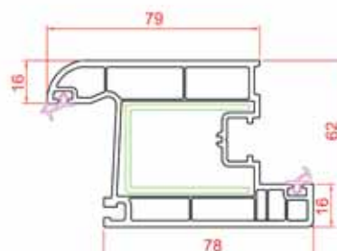
Narrow Door Sash
