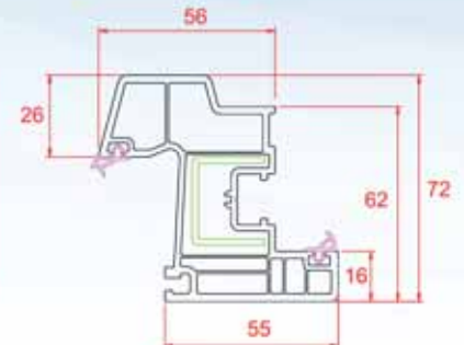
Drip Window Sash
