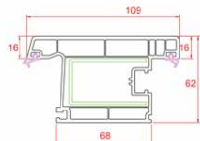
Outward Door Sash
