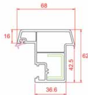
Lap Profile
