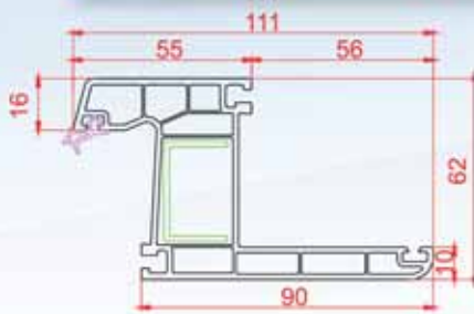
Super Architrave Frame
