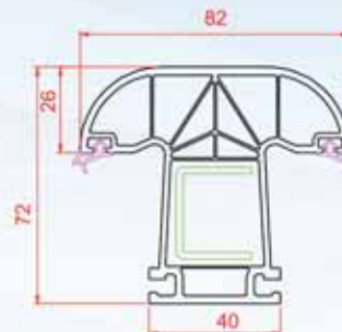
Mullion
