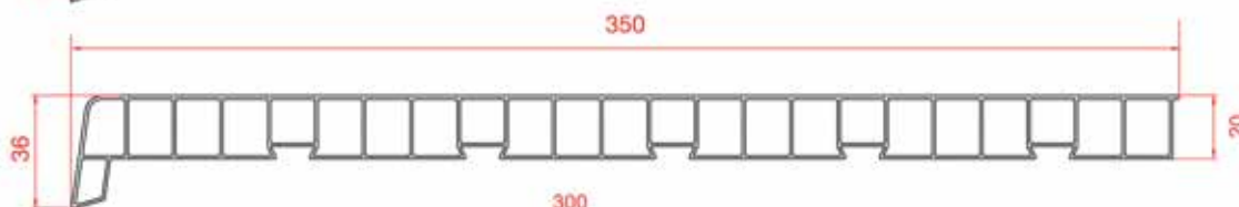
350 mm Window Sill
