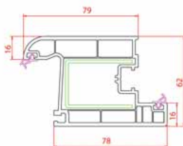
Narrow Door Sash
