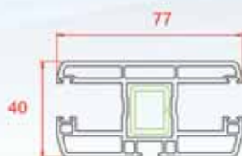
Mullion Rail Guide Profile
