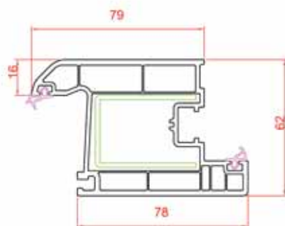
Narrow Door Sash
