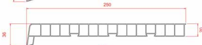
250 mm Window Sill
