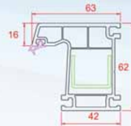
Frame
