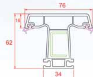
Narrow Mullion
