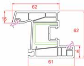
Super Window Sash
