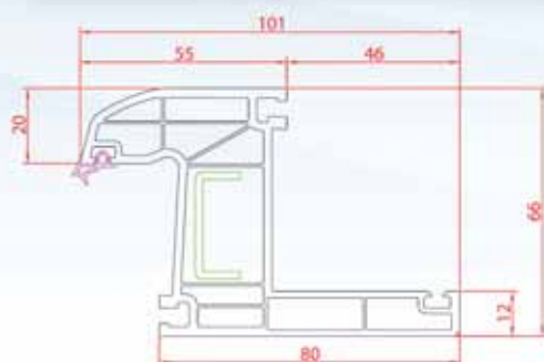
Architrave Frame
