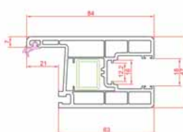
Window Sash
