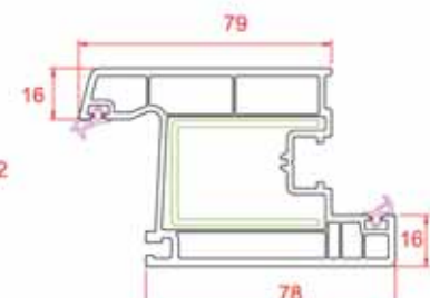
Narrow Door Sash
