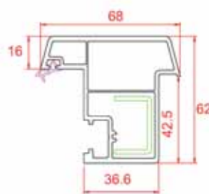
Lap Profile
