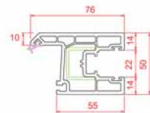
Window Sash
