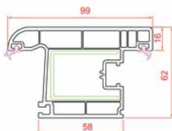
Narrow Outward Door Sash
