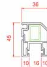
Fly Screen Sash
