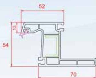
Architrave Frame
