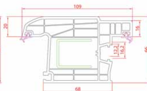
Outward Door Sash
