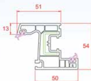
Narrow Window Sash
