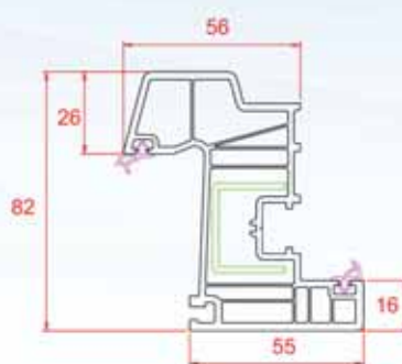
Drip Window Sash
