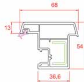
Lap Profile
