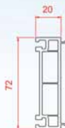
72 mm 2 cm Extension
