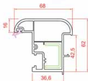
Lap Profile
