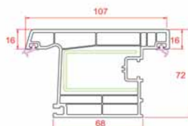
Outward Door Sash
