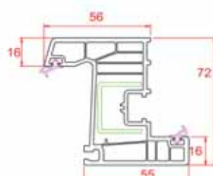
Window Sash
