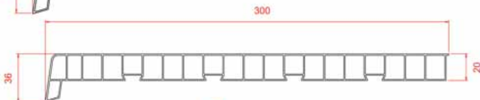
300 mm Window Sill
