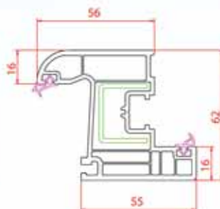
Window Sash
