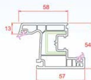
Window Sash
