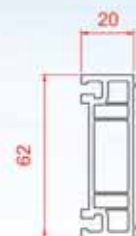
62 mm 2 cm Extension
