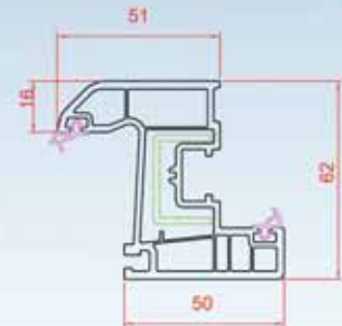
Narrow Window Sash
