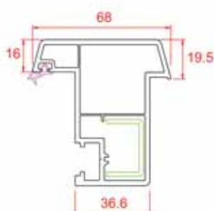
Lap Profile
