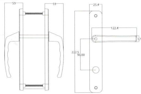
AKK20 Alüminyum WC Kapı Kolu Dar Ayna ELIT Aluminium Wc Door Handle Narrow Type ELIT 000000 ELIT
