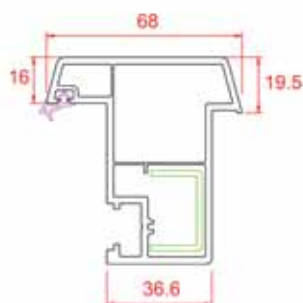
Lap Profile
