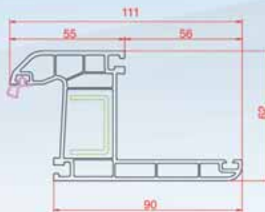
Super Architrave Frame
