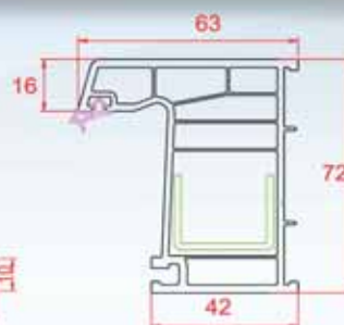
Frame
