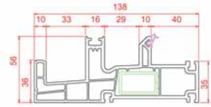
Single Frame With Fly Screen
