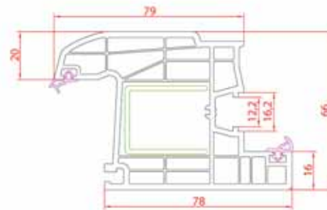
Narrow Door Sash
