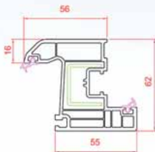
Window Sash
