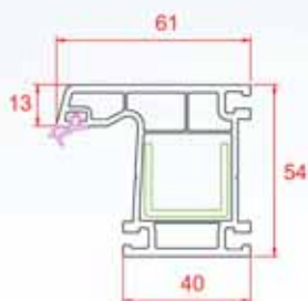
Frame
