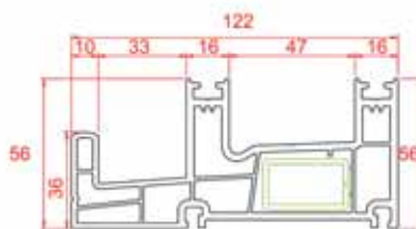
Double Frame With Fly Screen
