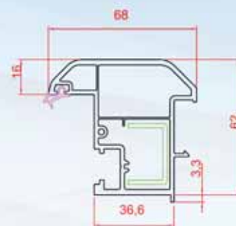
Lap Profile
