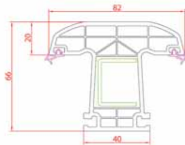
Mullion
