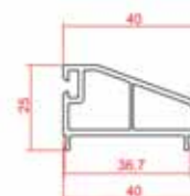
Side Cover
