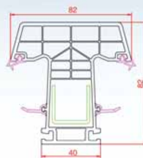
Mullion
