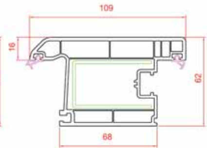
Outward Door Sash
