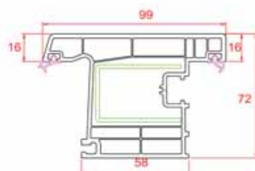
Narrow Outward Door Sash
