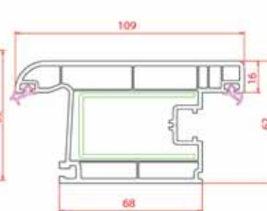
Outward Door Sash
