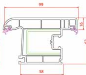
Narrow Outward Door Sash
