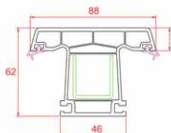
Super Mullion
