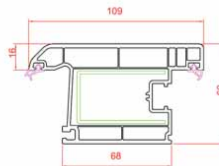
Outward Door Sash
