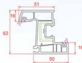
Narrow Window Sash
