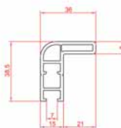
Fly Screen Rail
