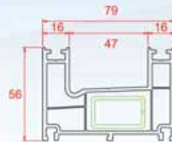
Double Frame
