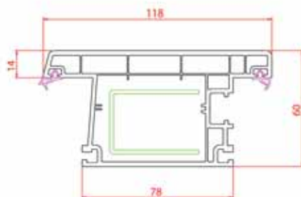
Outward Door Sash
