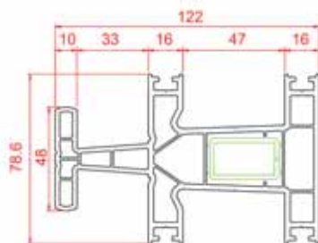
Frame Mullion
