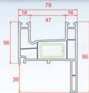
Architrave Double Frame
