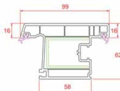
Narrow Outward Door Sash
