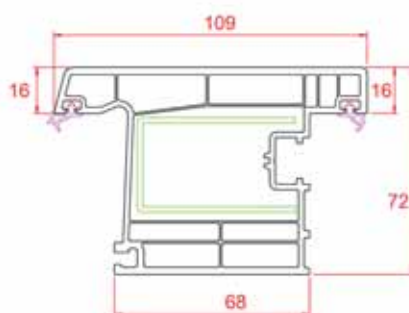
Outward Door Sash
