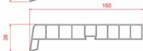
150 mm Window Sill
