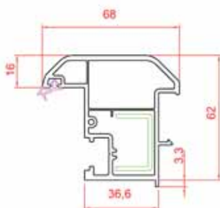
Lap Profile
