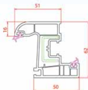
Narrow Window Sash
