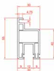
Fly Screen Sash
