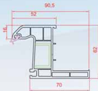
Architrave Frame
