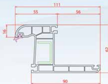
Super Architrave Frame
