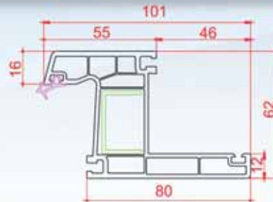
Architrave Frame
