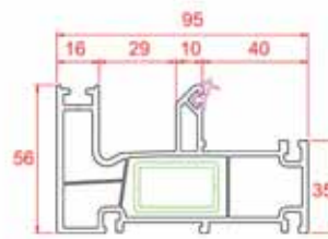
Single Frame
