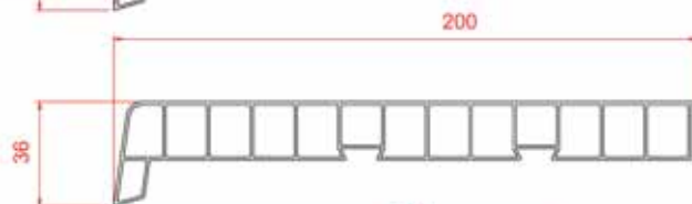
200 mm Window Sill
