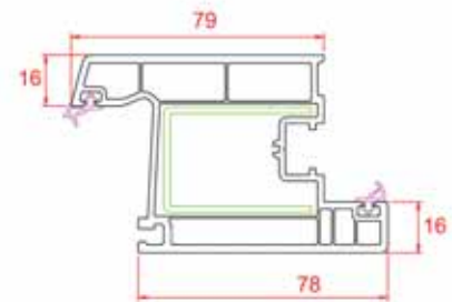
Narrow Door Sash
