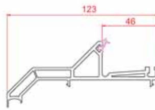
Frame Mullion Adaptor
