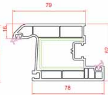
Narrow Door Sash
