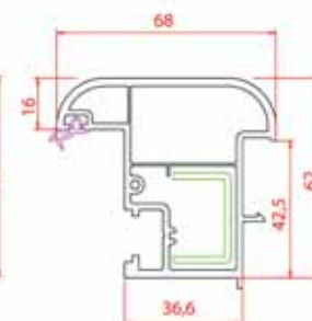
Lap Profile
