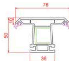
Mullion
