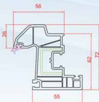
Drip Window Sash
