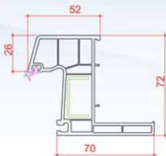
Architrave Frame
