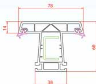
Mullion
