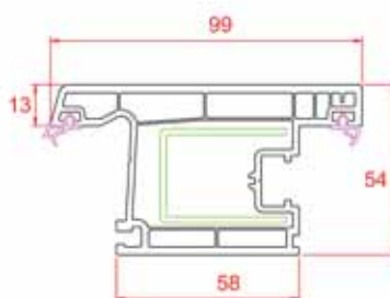
Outward Door Sash
