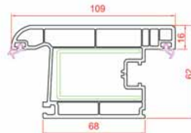
Outward Door Sash
