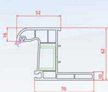
Architrave Frame
