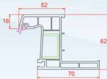
Architrave Frame
