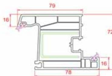
Narrow Door Sash
