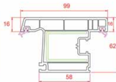
Narrow Outward Door Sash
