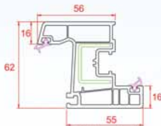
Window Sash
