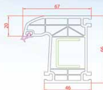
Super Frame
